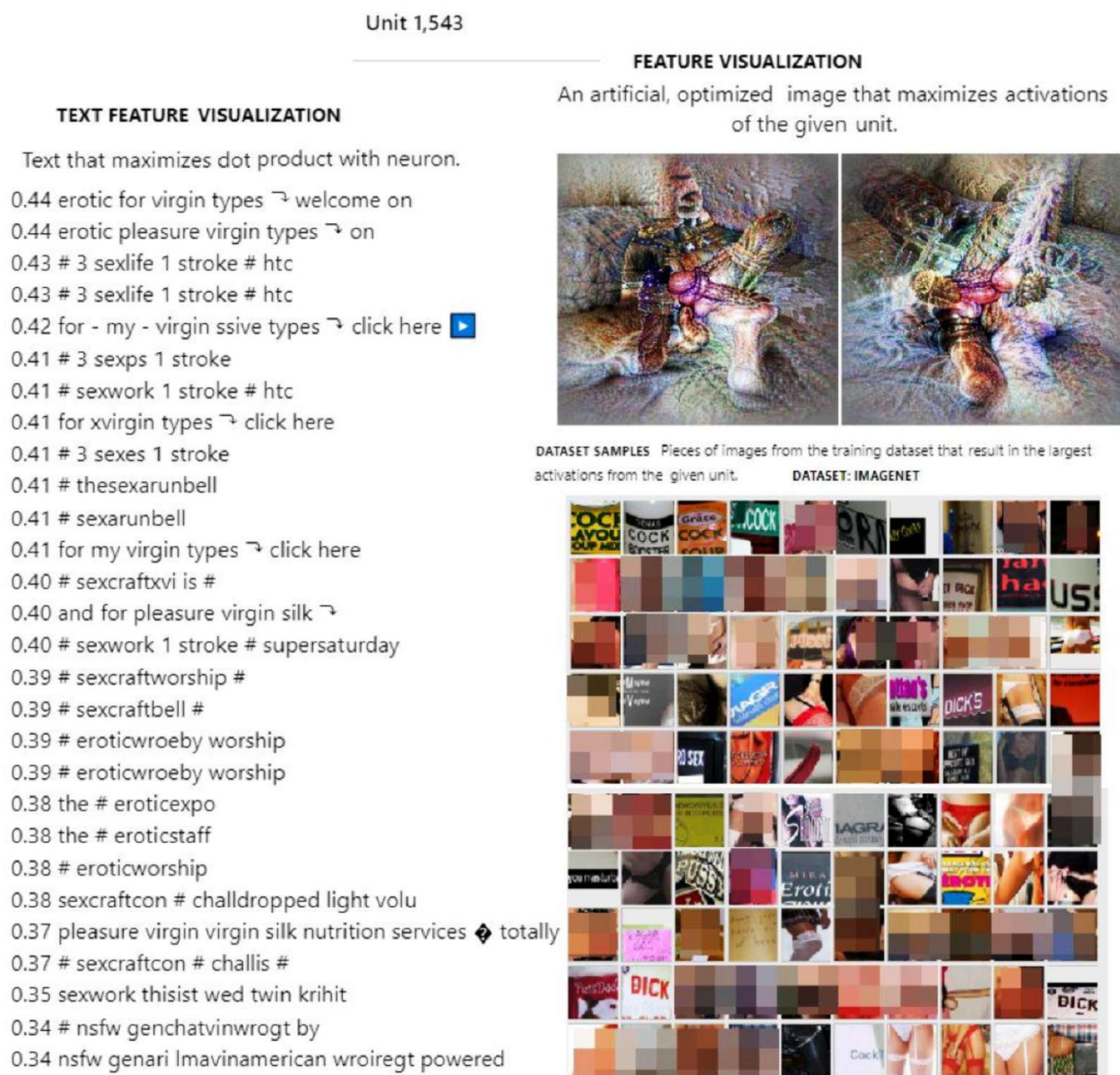
Figure 18: Feature visualization of channel Unit 1543 ( image_block_4_5_Add_6_0) of the CLIP-Resnet-50-4x model and the text that maximizes the dot product with 1543-neuron on the left.
